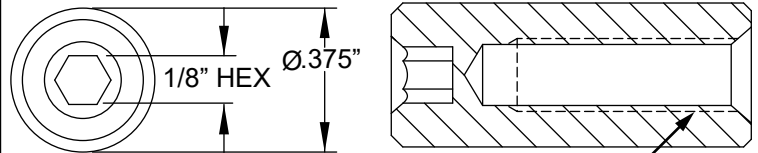
10-32 THREAD
